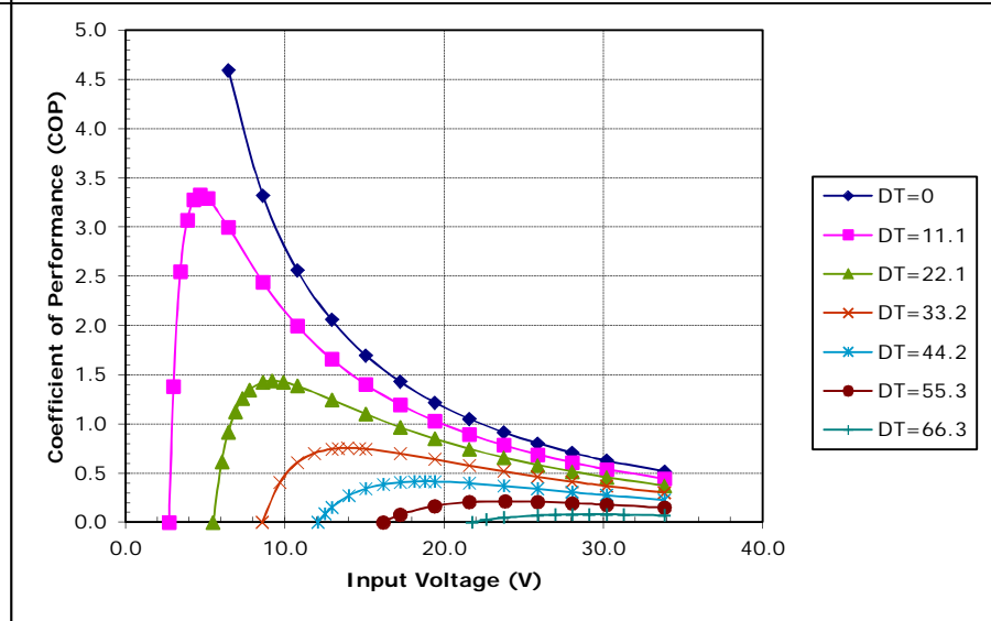
Potted RD-253-1.4-1.5 at a hot-side temperature of 50 °C
