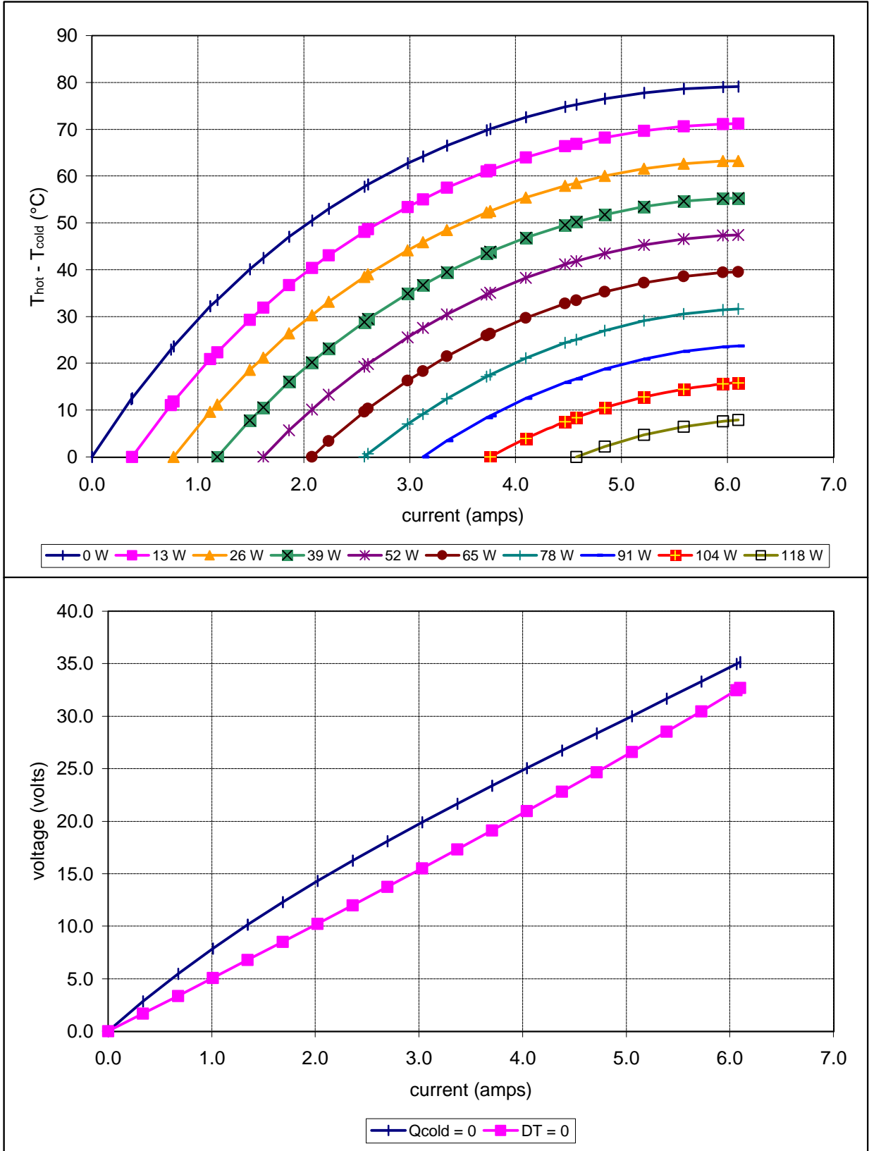
Unpowered RD-253-1.4-1.5 at a hot-side temperature of 50 °C
