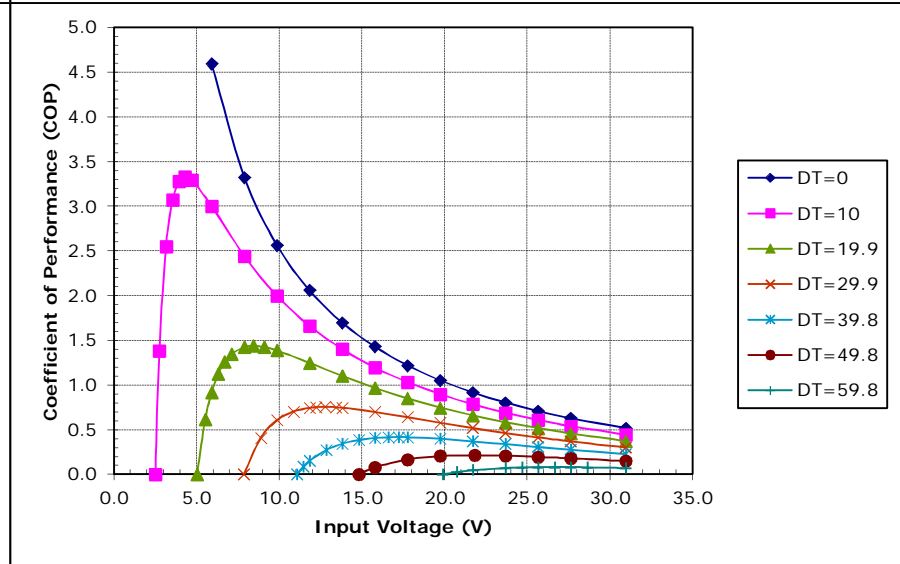
Potted RD-253-1.4-1.5 at a hot-side temperature of 30 °C
