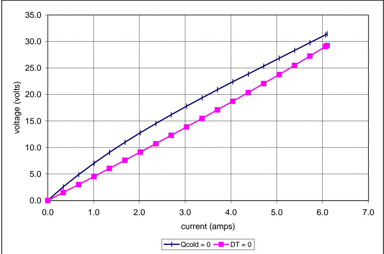
Unpotted RD-253-1.4-1.5 at a hot-side temperature of 25 °C
