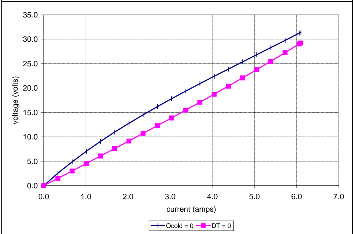
Potted RD-253-1.4-1.5 at a hot-side temperature of 25 °C
