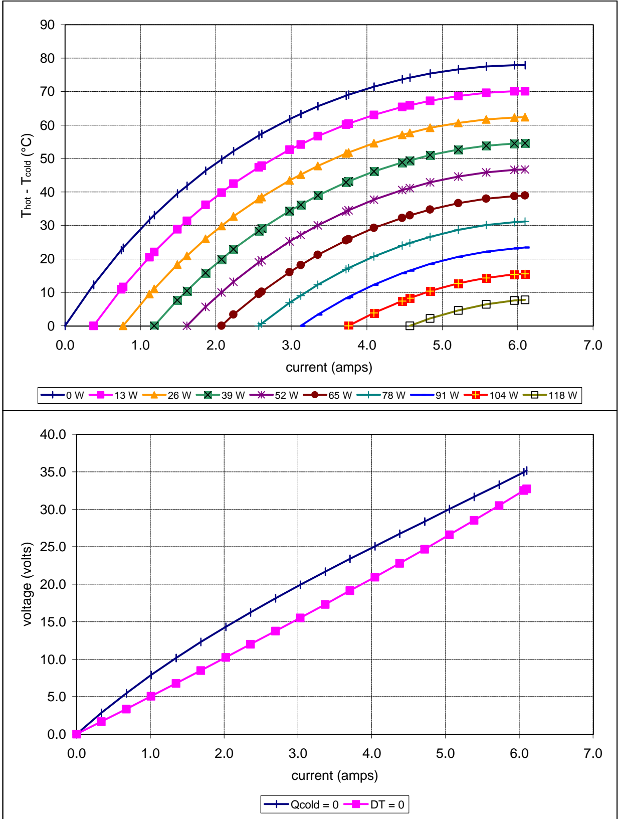
Potted RD-253-1.4-1.5 at a hot-side temperature of 50 °C
