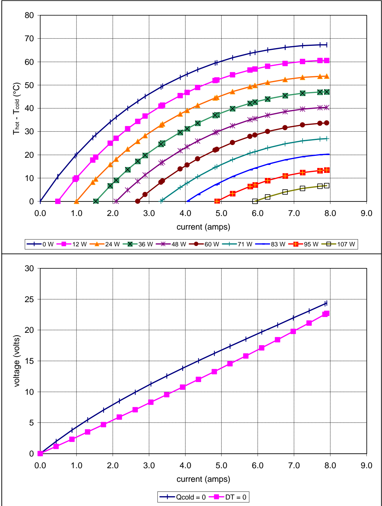
Potted HP-199-1.4-1.15 at a hot-side temperature of 25 °C
