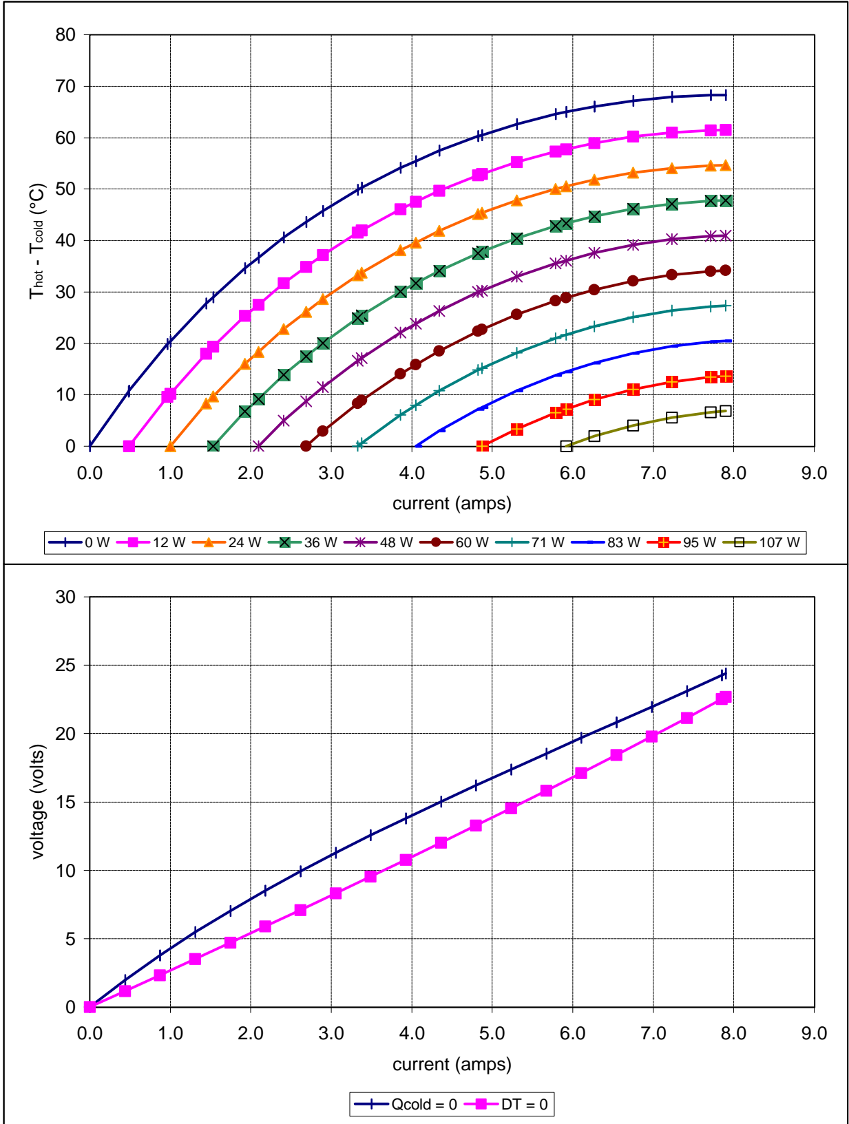
Unpotted HP-199-1.4-1.15 at a hot-side temperature of 25 °C
