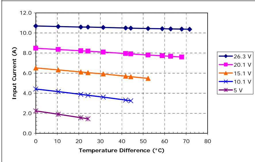
Potted HP-199-1.4-0.8 at a hot-side temperature of 50 °C
