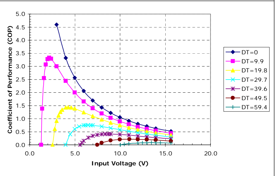
Potted HP-127-1.4-2.5-72 at a hot-side temperature of 30 °C
