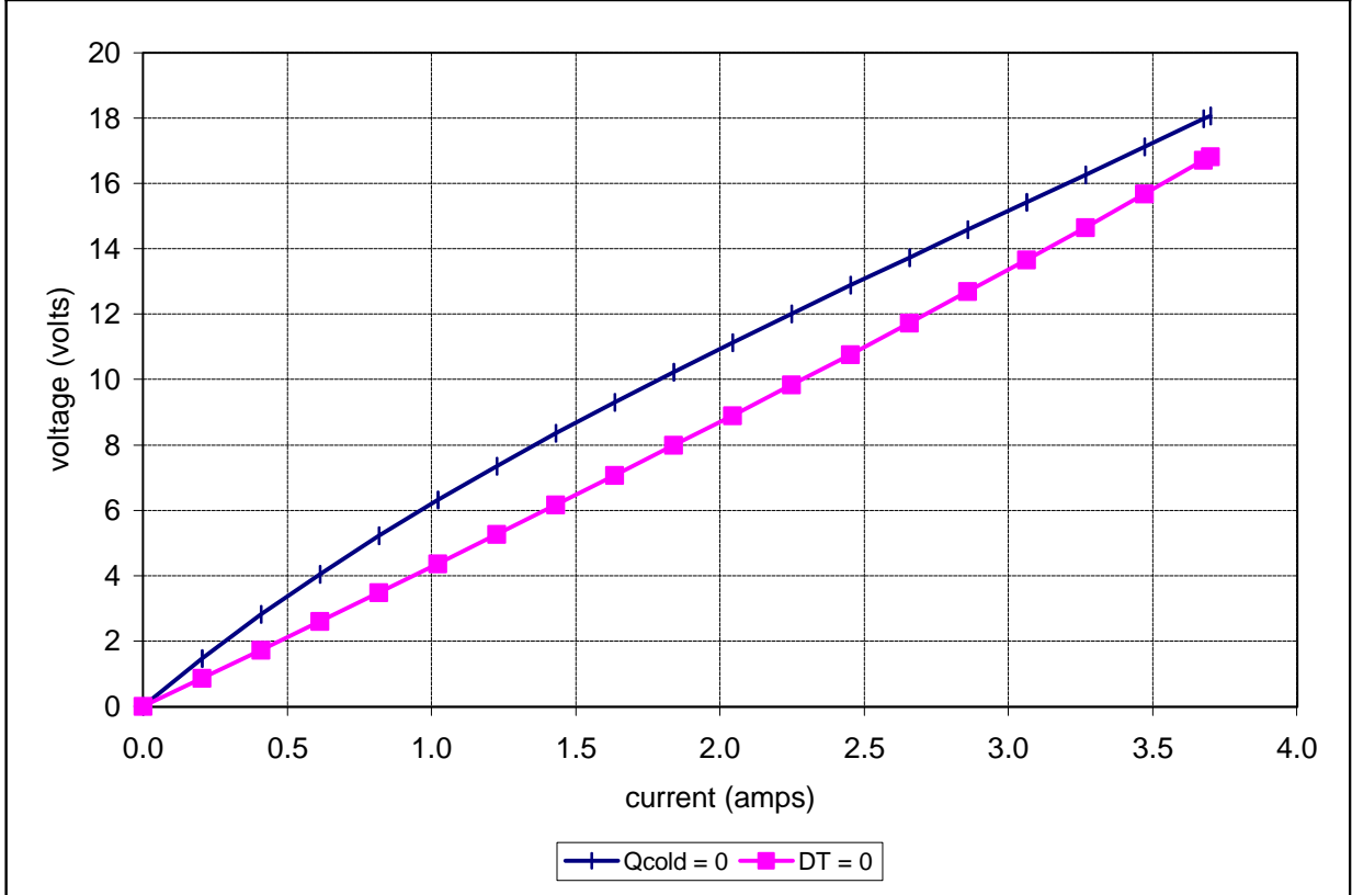
Unpotted HP-127-1.4-2.5-72 at a hot-side temperature of 50 °C
