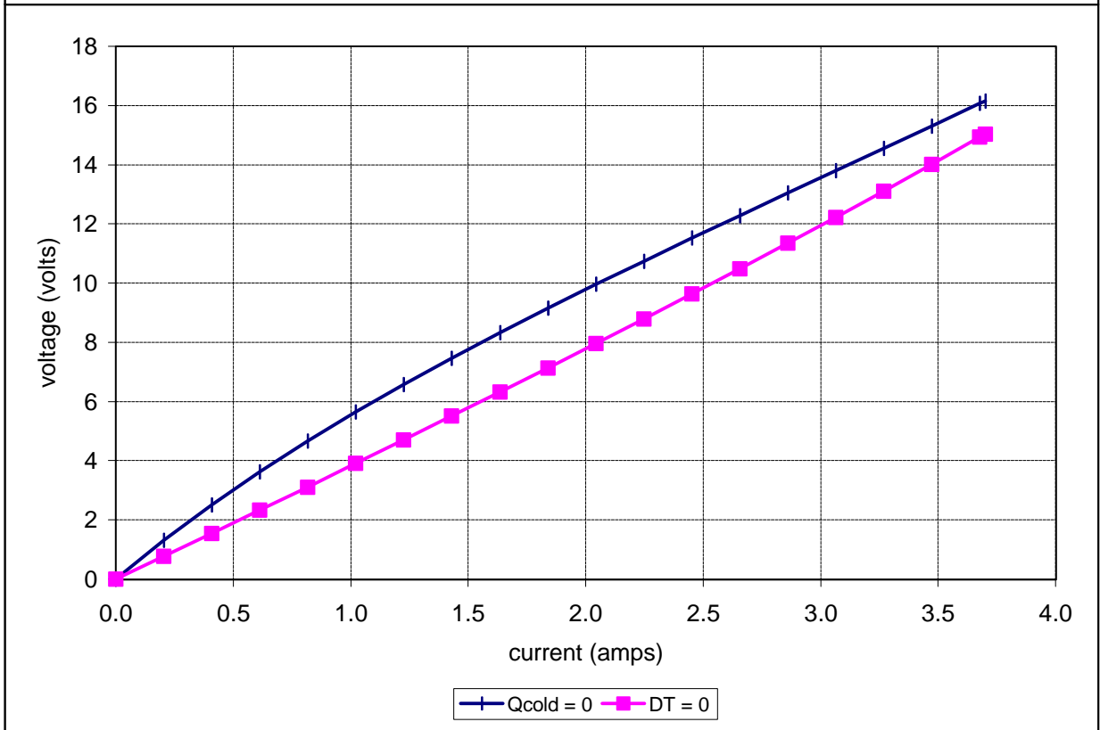
Potted HP-127-1.4-2.5-72 at a hot-side temperature of 25 °C
