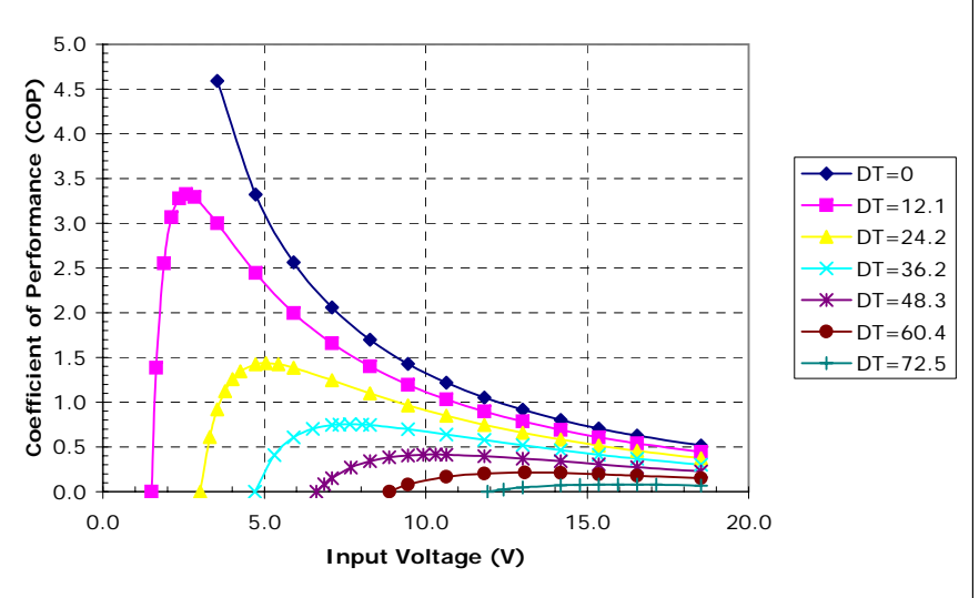
Potted HP-127-1.4-2.5-72 at a hot-side temperature of 70 °C
