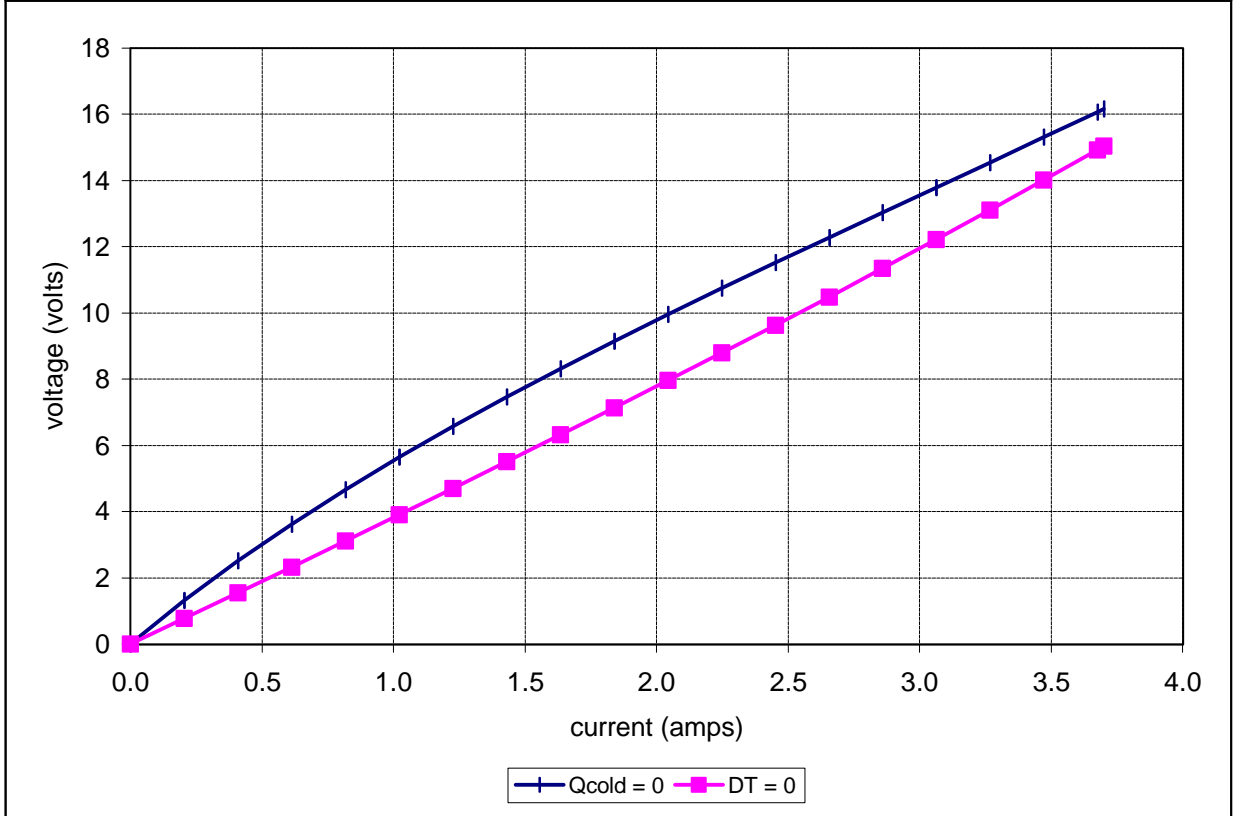
Unpotted HP-127-1.4-2.5-72 at a hot-side temperature of 25 °C
