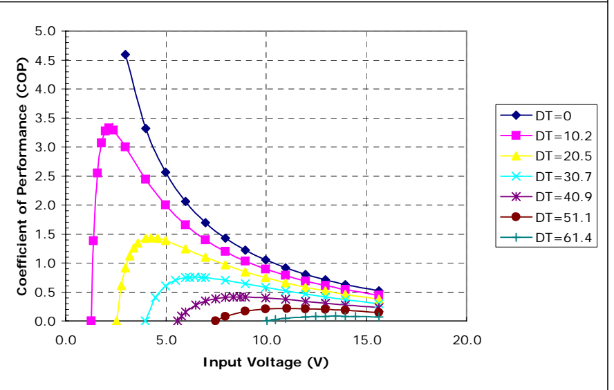
Unpotted HP-127-1.4-2.5-72 at a hot-side temperature of 30 °C
