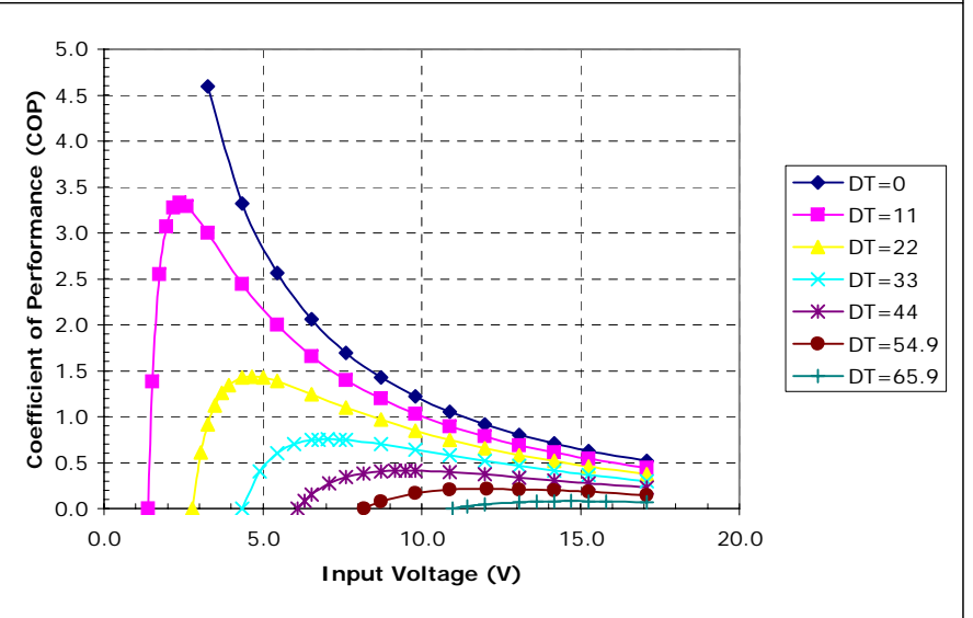
Potted HP-127-1.4-2.5-72 at a hot-side temperature of 50 °C
