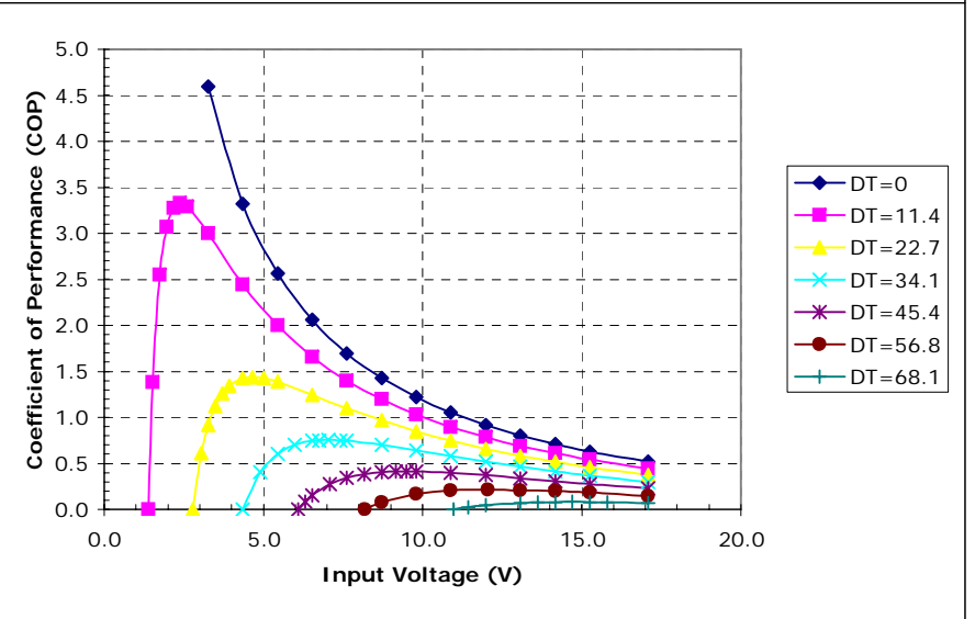
Unpotted HP-127-1.4-2.5-72 at a hot-side temperature of 50 °C
