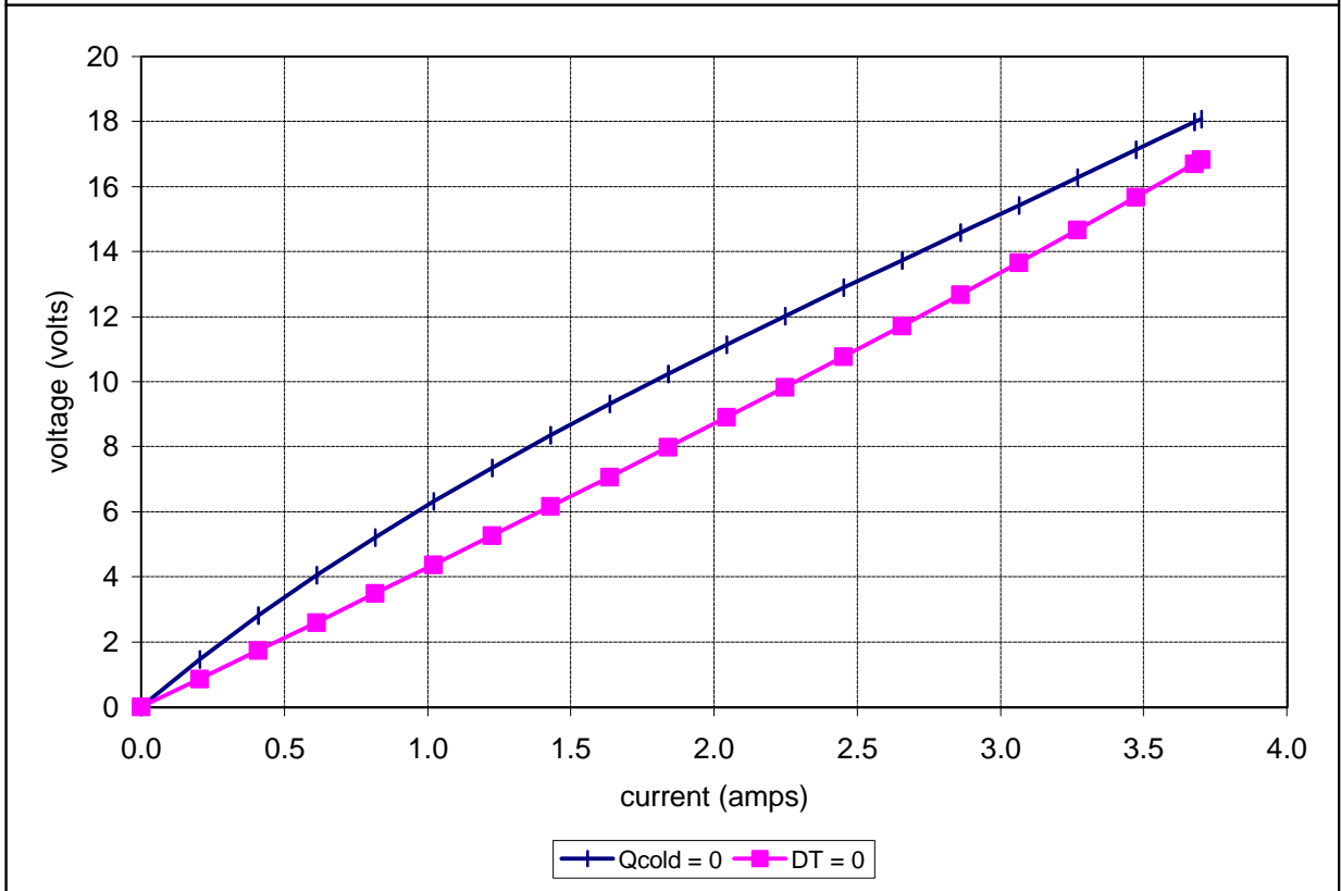
Potted HP-127-1.4-2.5-72 at a hot-side temperature of 50 °C
