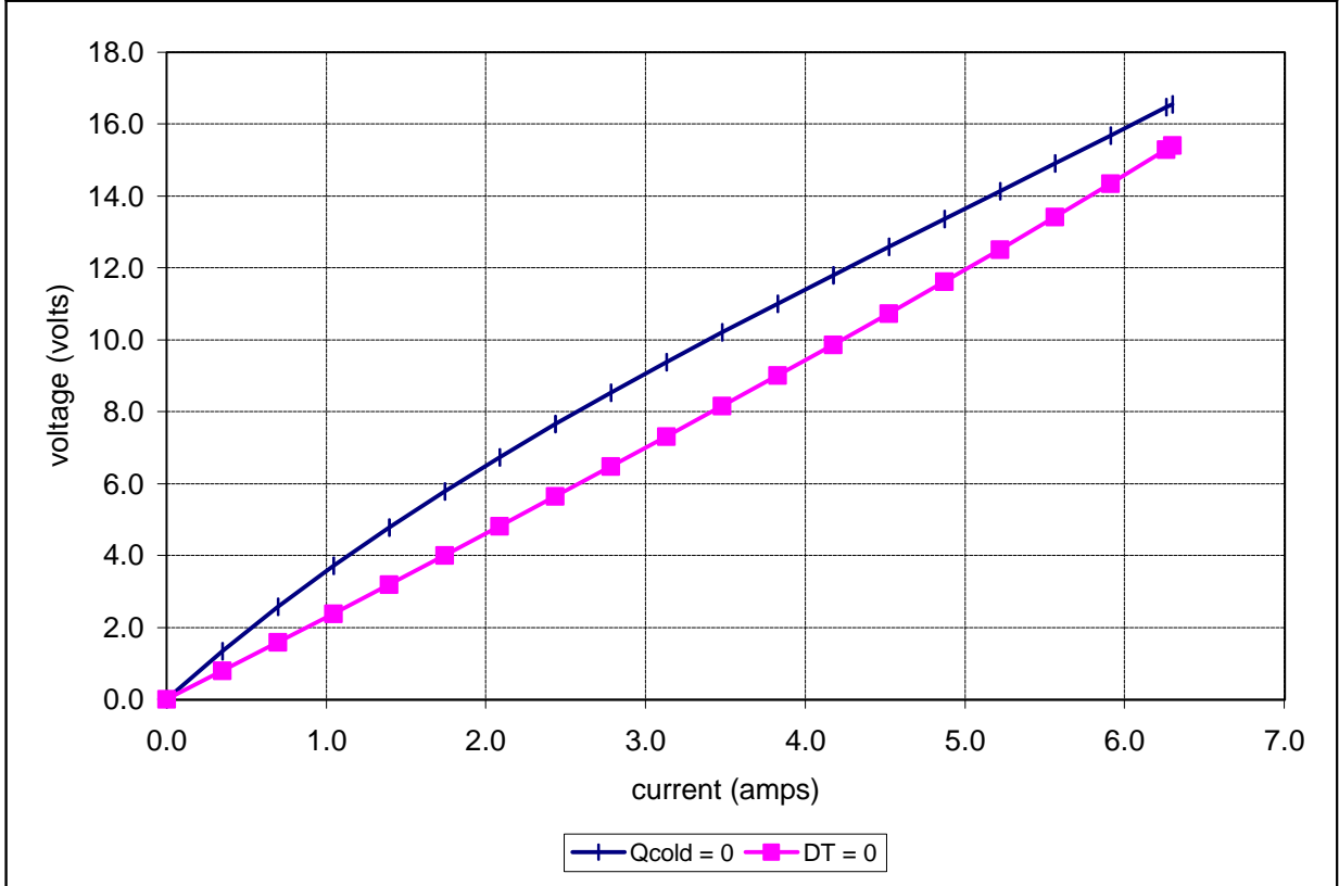
Unpotted HP-127-1.4-1.5-74 at a hot-side temperature of 25 °C
