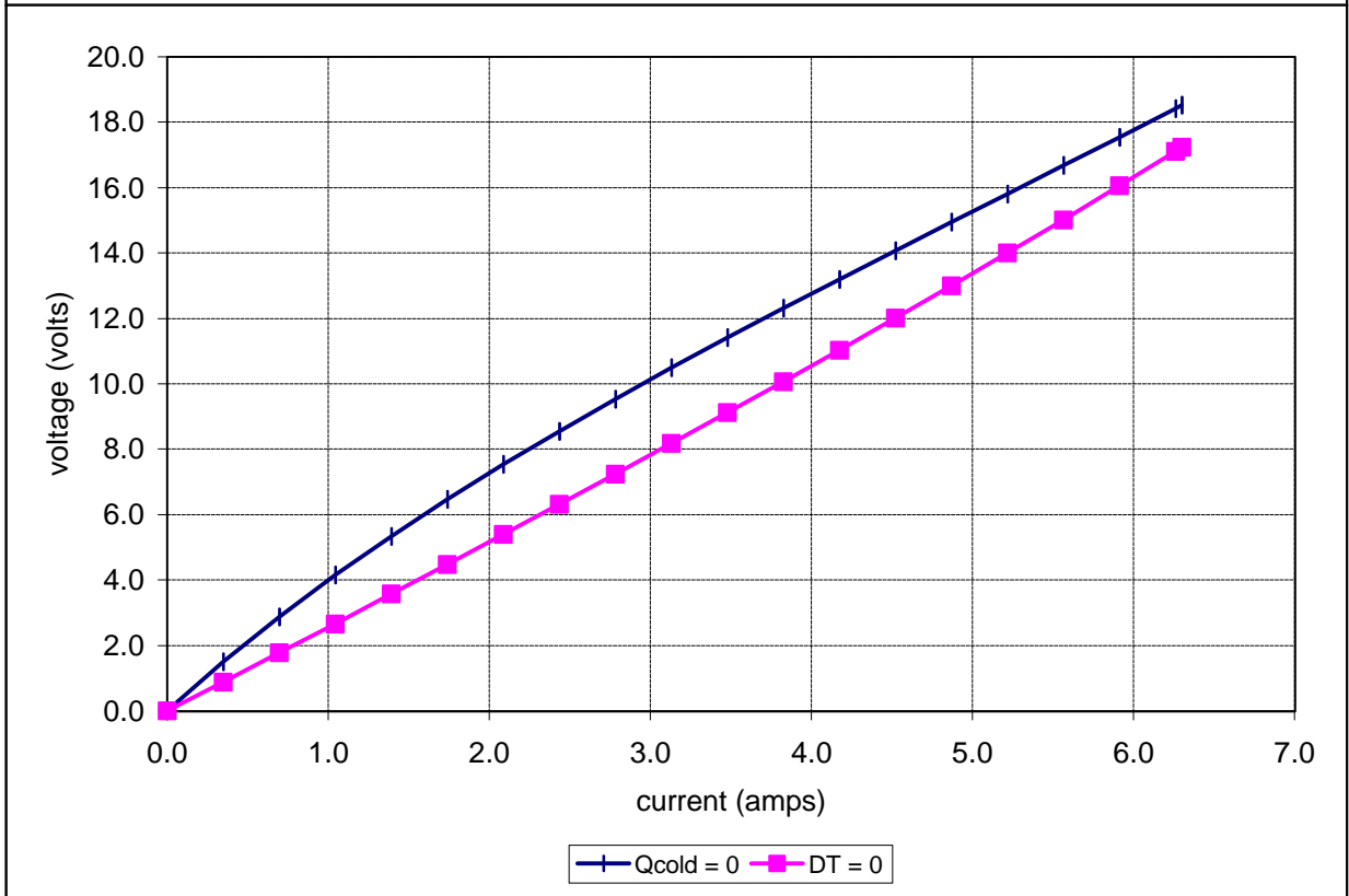
Potted HP-127-1.4-1.5-74 at a hot-side temperature of 50 °C
