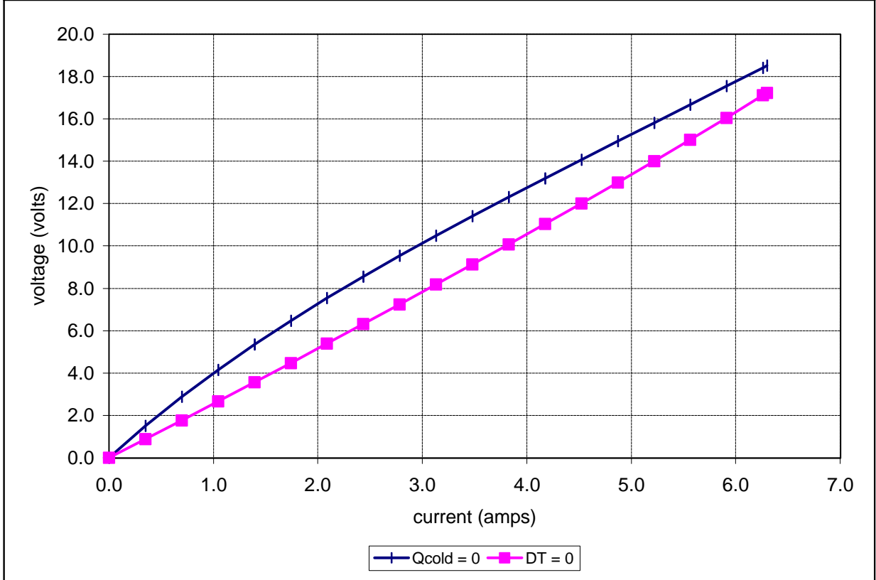
Unpotted HP-127-1.4-1.5-74 at a hot-side temperature of 50 °C
