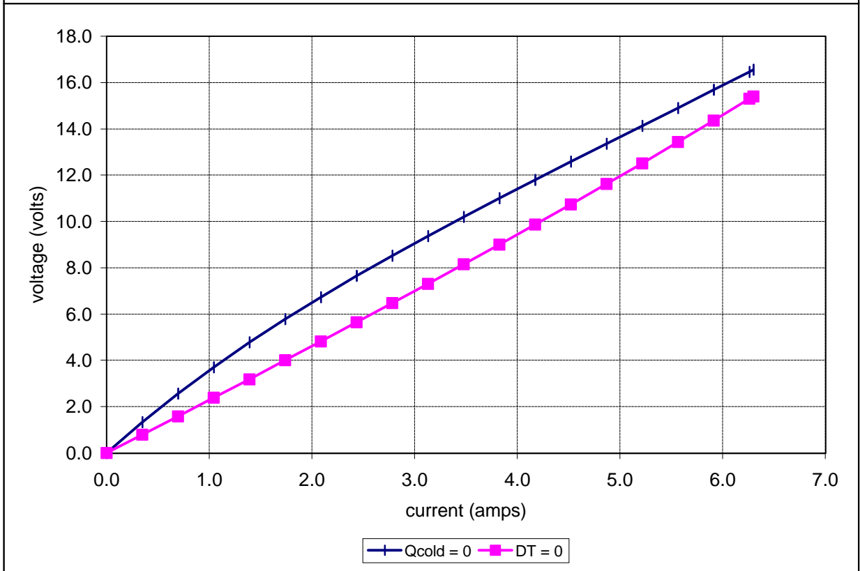
Potted HP-127-1.4-1.5-74 at a hot-side temperature of 25 °C
