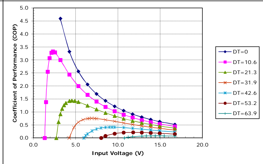
Potted HP-127-1.4-1.15-71 at a hot-side temperature of 50 °C
