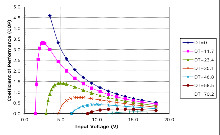
Potted HP-127-1.4-1.15-71 at a hot-side temperature of 70 °C
