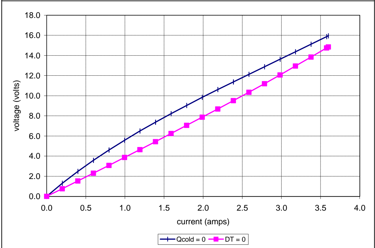
Unpotted HP-127-1.0-1.3-71 at a hot-side temperature of 25 °C
