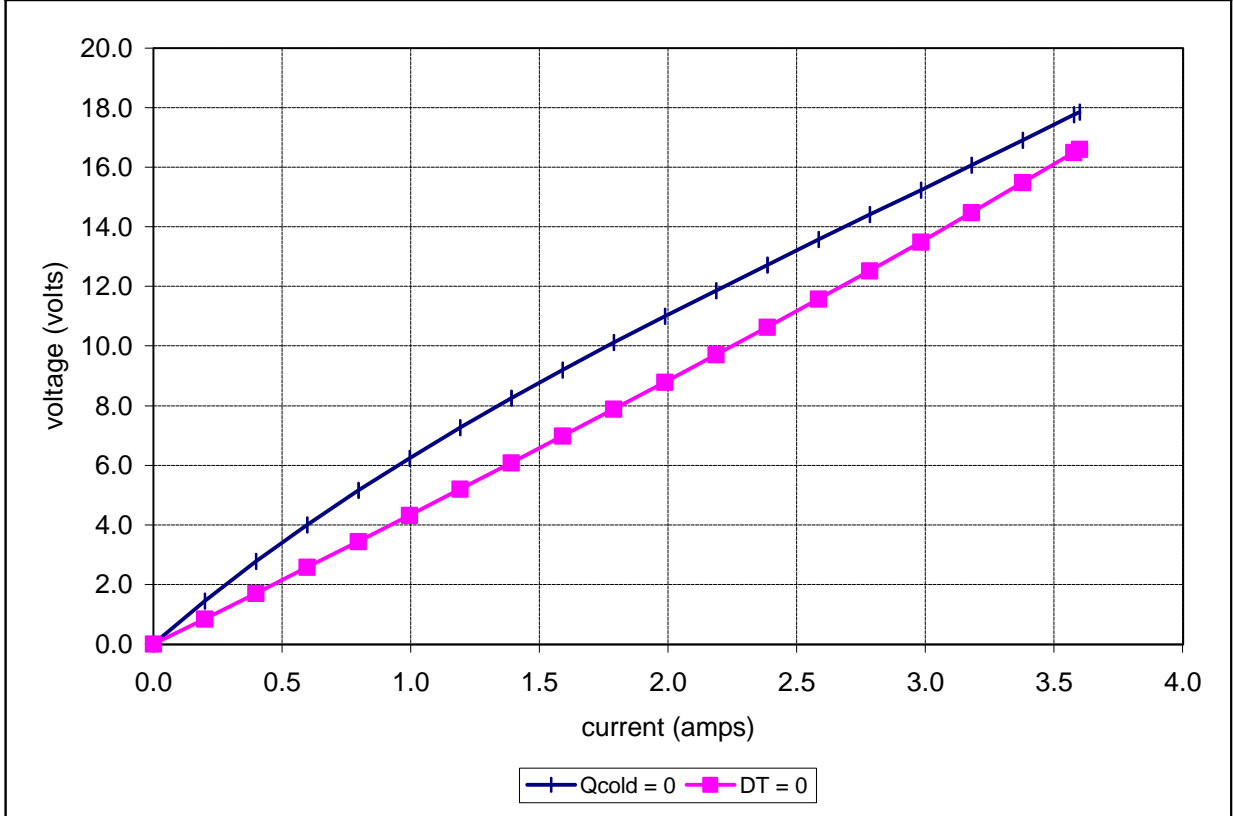
Unpotted HP-127-1.0-1.3-71 at a hot-side temperature of 50 °C
