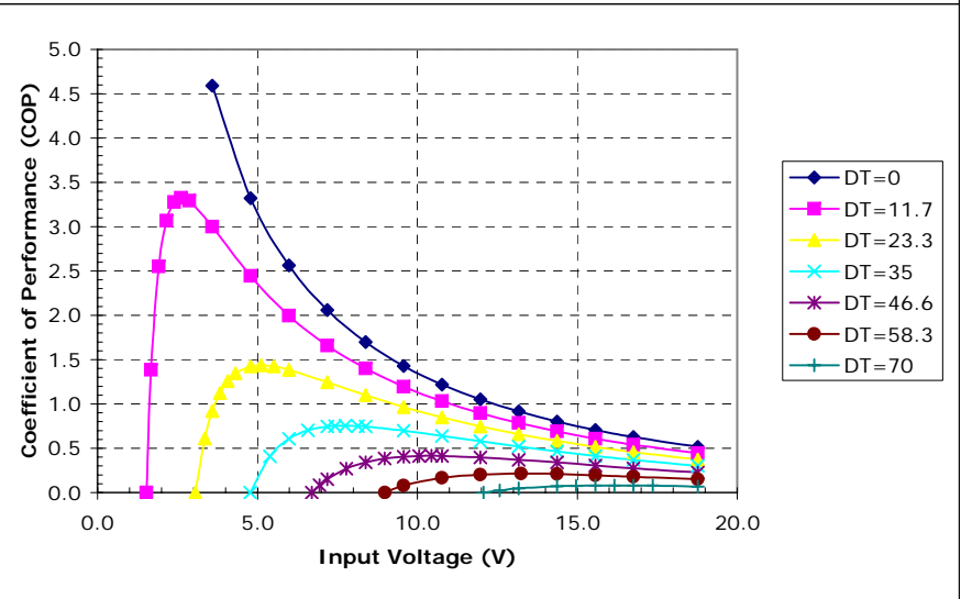
Potted HP-127-1.0-1.3-71 at a hot-side temperature of 70 °C
