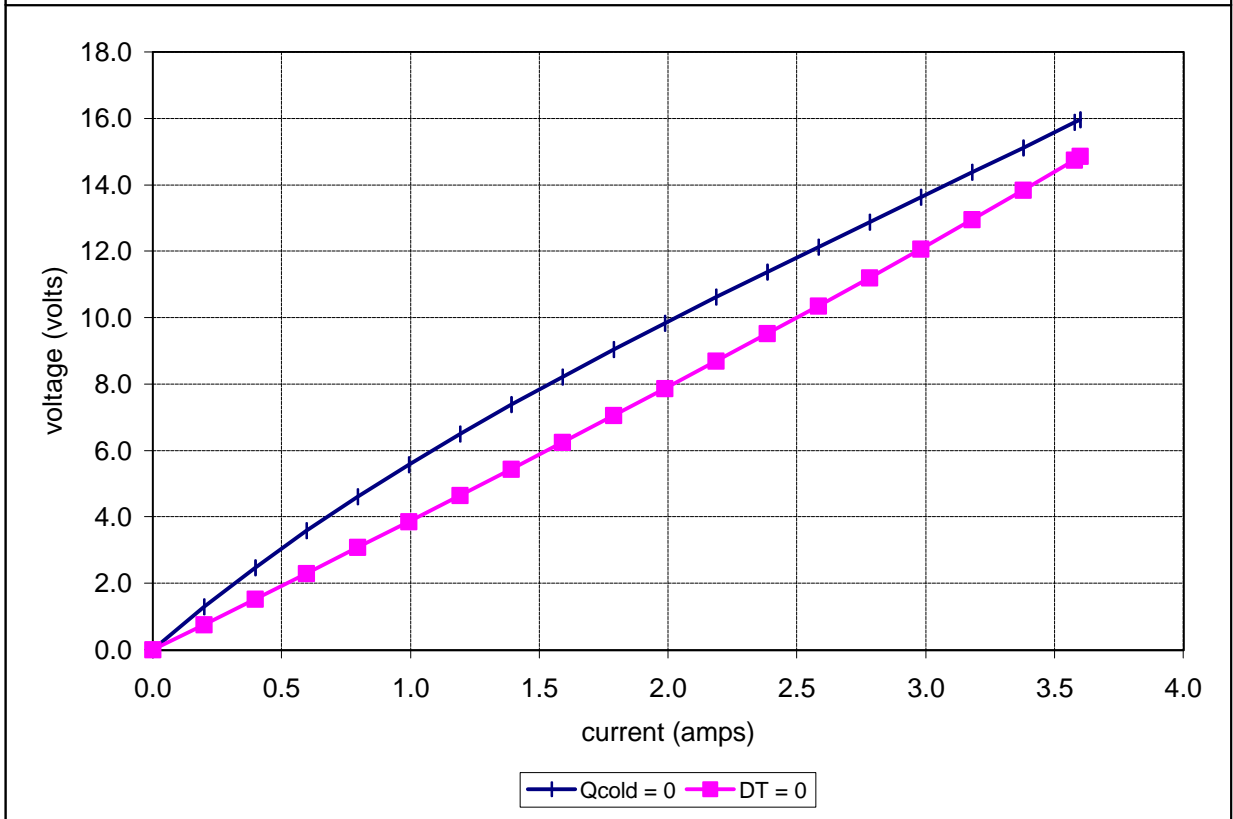
Potted HP-127-1.0-1.3-71 at a hot-side temperature of 25 °C
