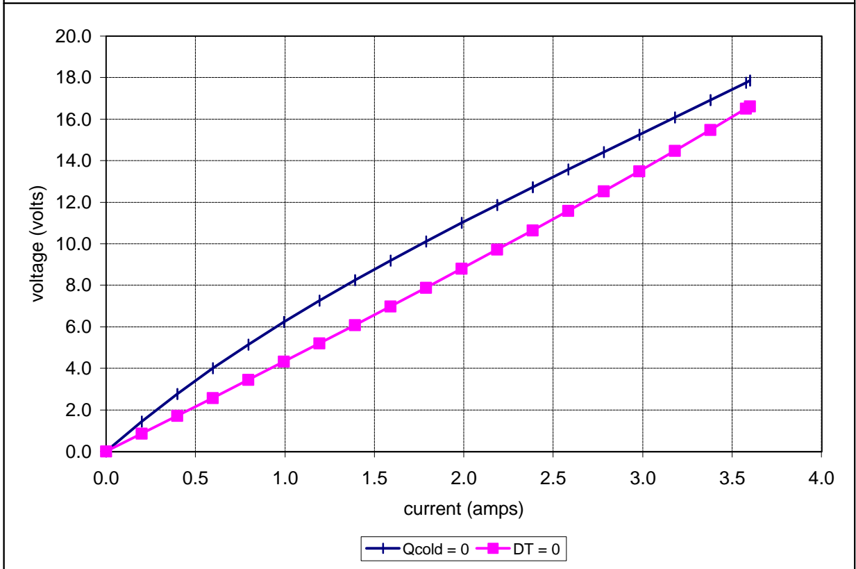
Potted HP-127-1.0-1.3-71 at a hot-side temperature of 50 °C
