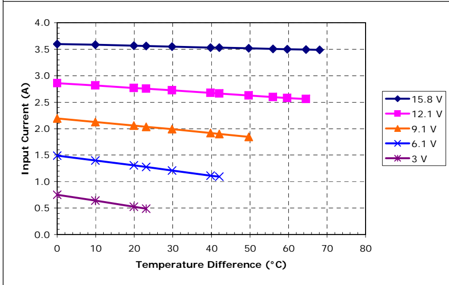
Unpotted HP-127-1.0-1.3-71 at a hot-side temperature of 30 °C
