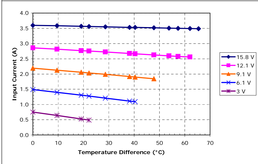
Potted HP-127-1.0-1.3-71 at a hot-side temperature of 30 °C
