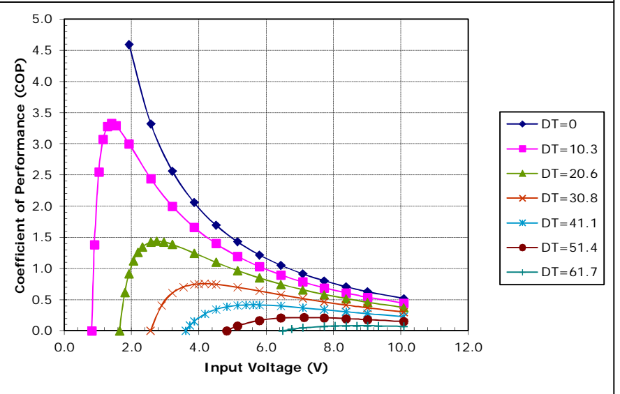
Unpotted CH-77-1.0-0.8 at a hot-side temperature of 50 °C
