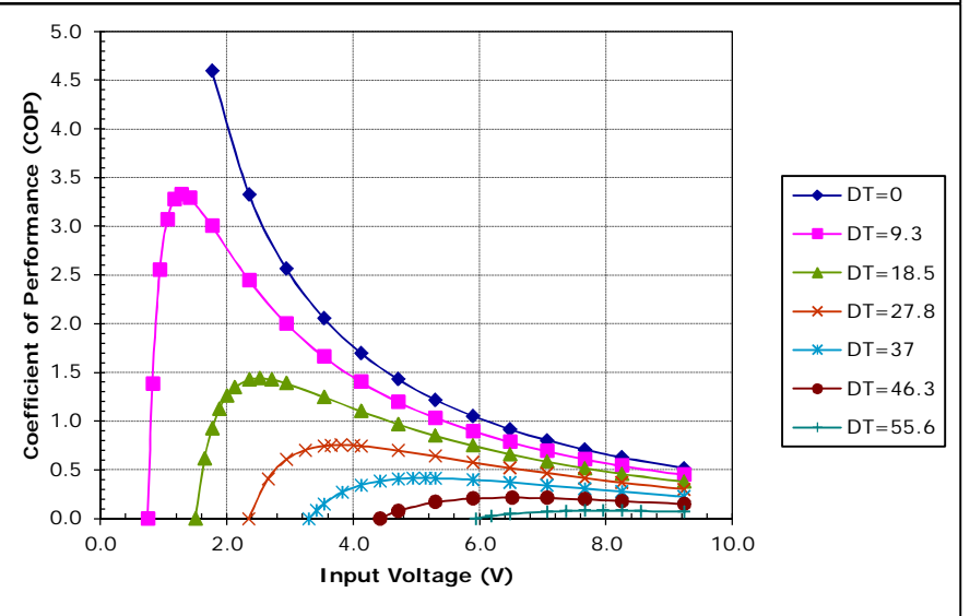
Unpotted CH-77-1.0-0.8 at a hot-side temperature of 30 °C
