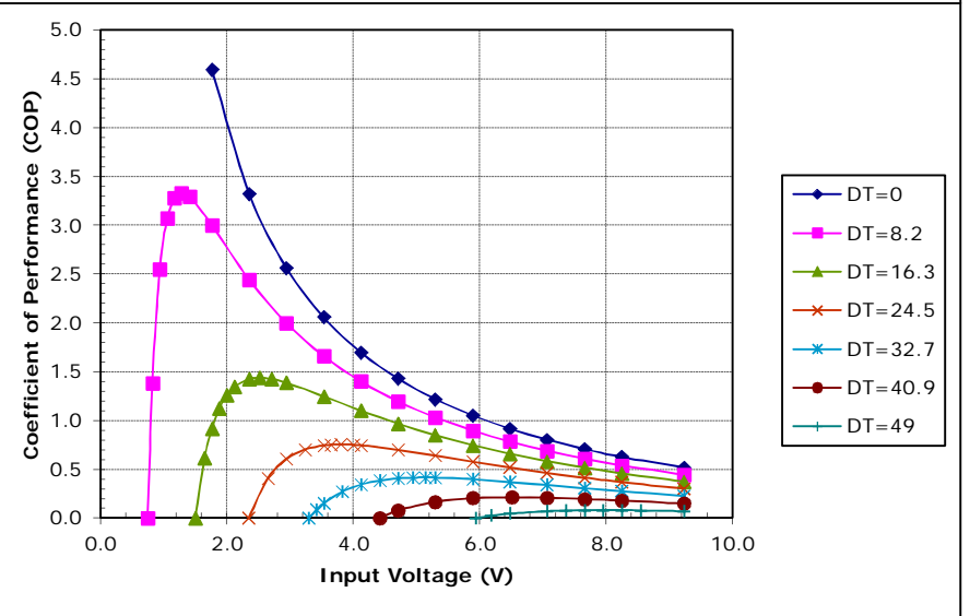
Potted CH-77-1.0-0.8 at a hot-side temperature of 30 °C
