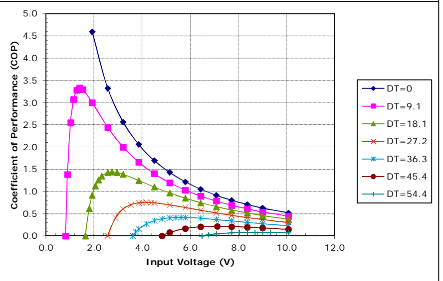
Potted CH-77-1.0-0.8 at a hot-side temperature of 50 °C
