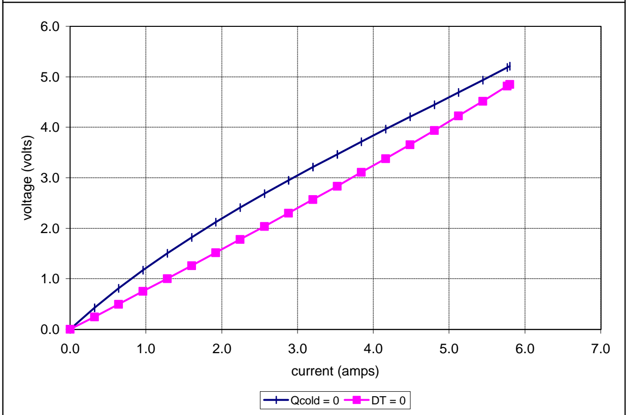
Potted CH-38-1.0-0.8 at a hot-side temperature of 50 °C
