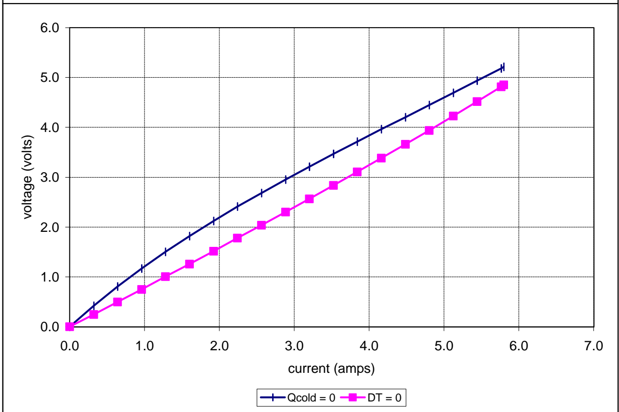
Unpotted CH-38-1.0-0.8 at a hot-side temperature of 50 °C
