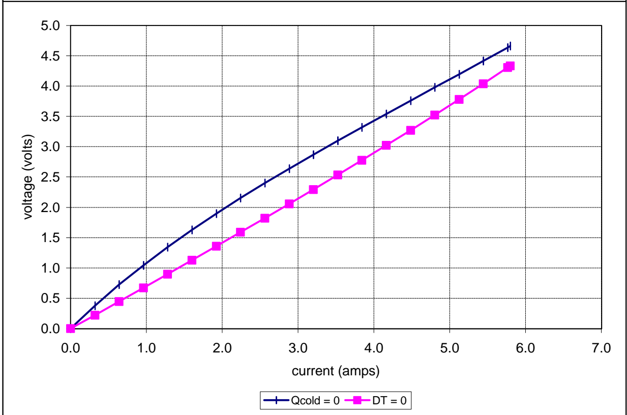
Unpotted CH-38-1.0-0.8 at a hot-side temperature of 25 °C
