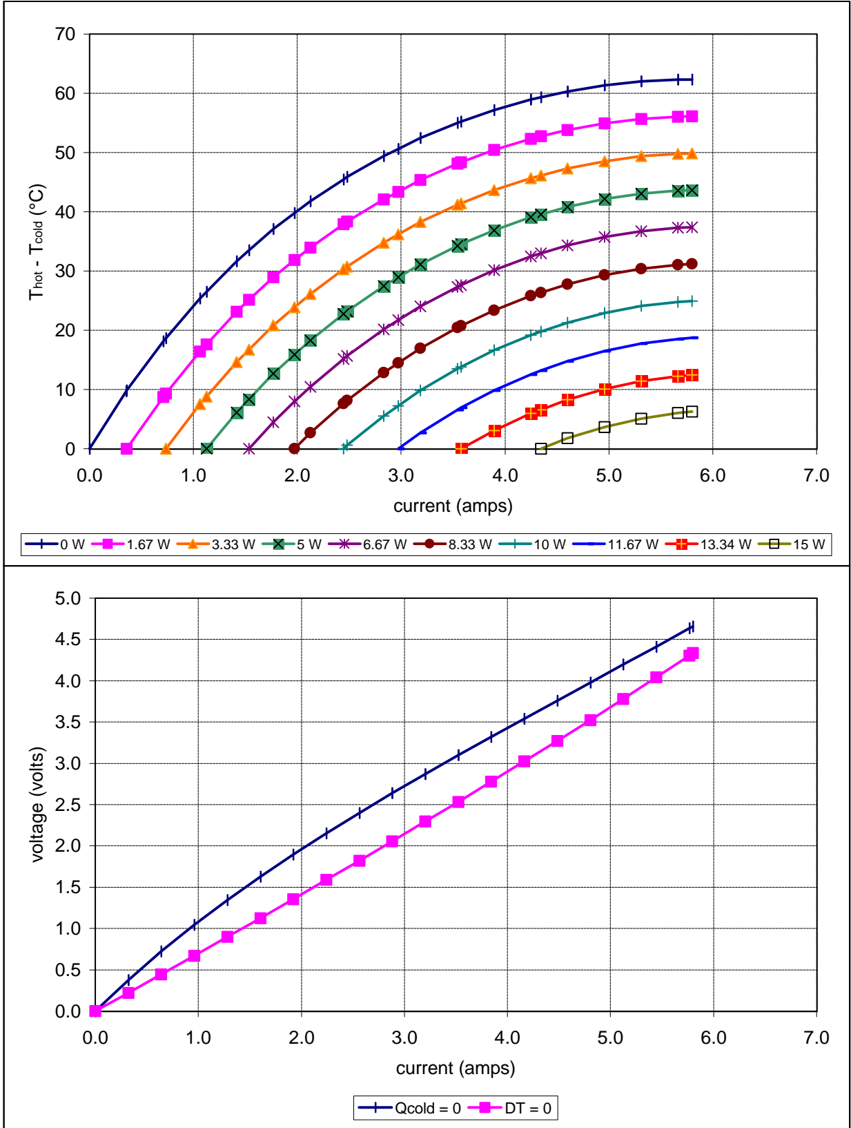
Potted CH-38-1.0-0.8 at a hot-side temperature of 25 °C
