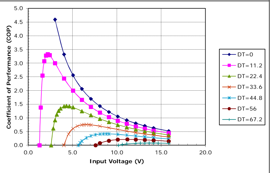
Unpotted CH-119-1.4-1.5 at a hot-side temperature of 50 °C
