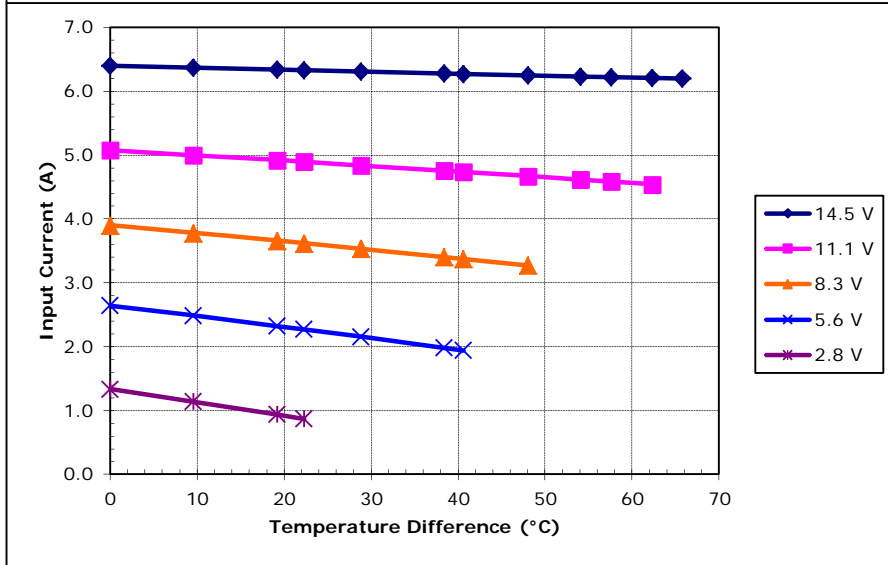
Potted CH-119-1.4-1.5 at a hot-side temperature of 30 °C
