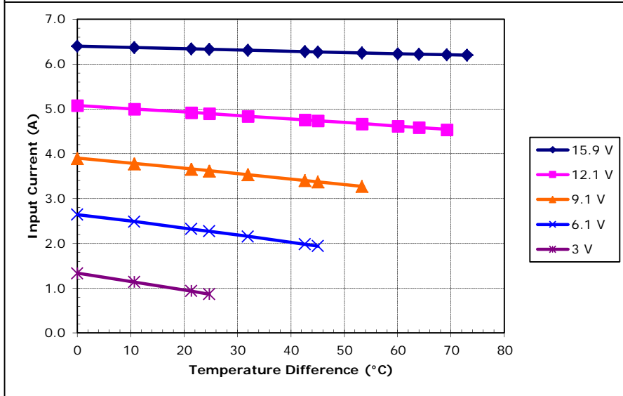
Potted CH-119-1.4-1.5 at a hot-side temperature of 50 °C
