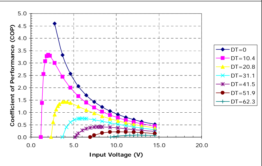
Potted CH-109-1.4-1.5 at a hot-side temperature of 50 °C
